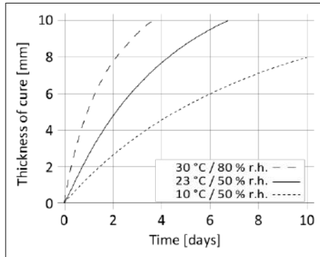
Diagram 1: Curing speed Sikaflex®-263 AP
